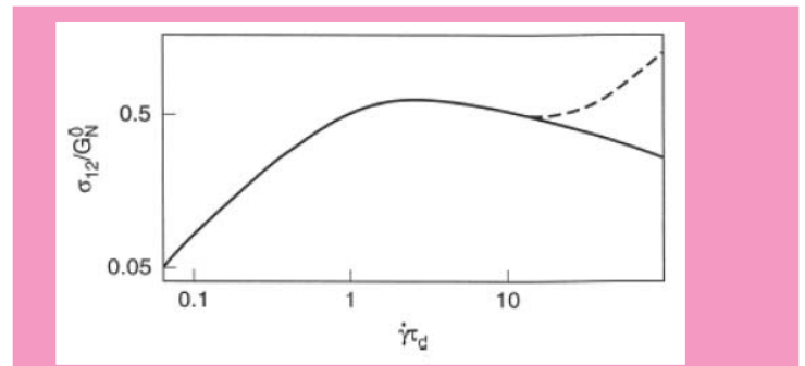
Figure 1: Dimensionless shear stress versus Wi based on the disengagement time as predicted by the Doi-Edwards theory (solid line). Dashed line adds a speculated contribution from Rouse modes. (Doi and Edwards [10]).
